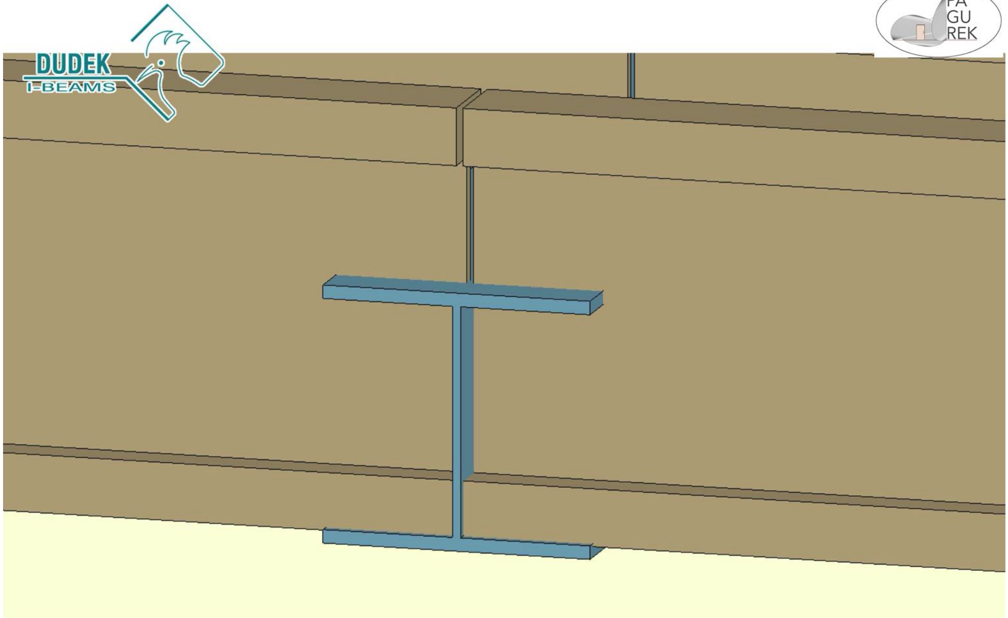
Connecting detail of timber I-beam
